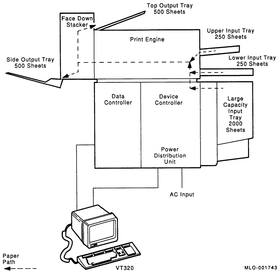
Figure 1-7 PrintServer 40 Series Hardware Components
